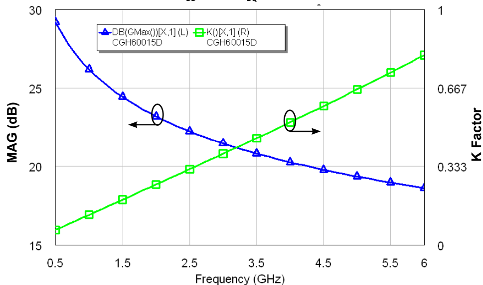
Simulated Maximum Available Gain and K Factor of the CGH60015D
