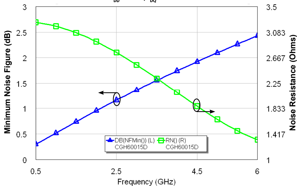
Simulated Minimum Noise Figure and Noise Resistance vs Frequency of the CGH60015D
