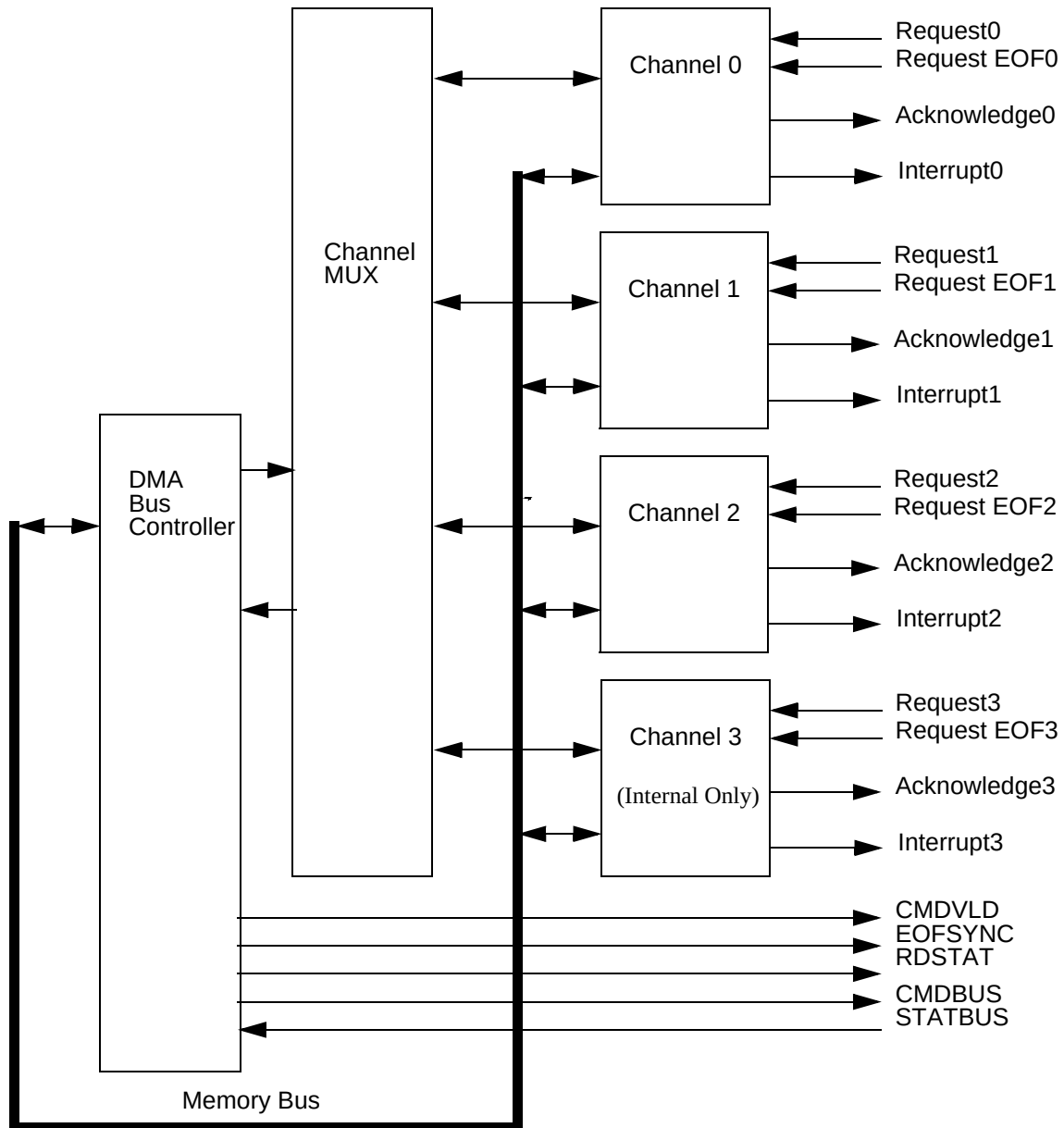
Figure 45. DMA Block Diagram
