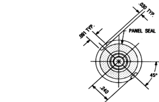
PANEL AND SHAFT SEAL
