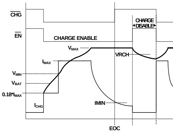
FIGURE 3. TIMING DIAGRAM
