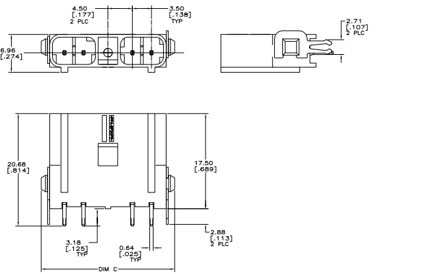
VERTICAL THRU HOLE HEADER
