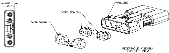
EXPLODED VIEW
