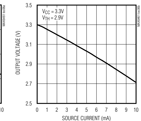
OUTPUT VOLTAGE HIGH vs. SOURCE CURRENT
