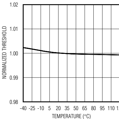
NORMALIZED THRESHOLD vs. TEMPERATURE
