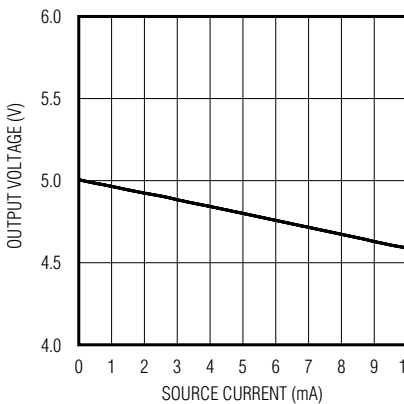
OUTPUT VOLTAGE HIGH vs. SOURCE CURRENT
