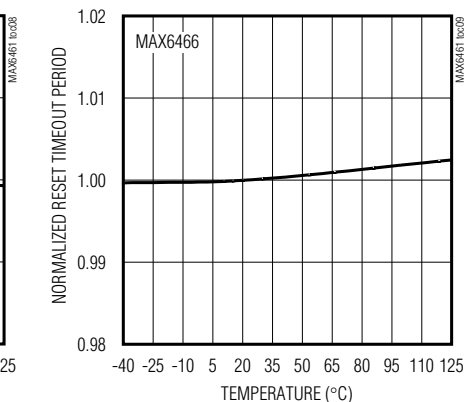
NORMALIZED OUTPUT TIMEOUT PERIOD vs. TEMPERATURE
