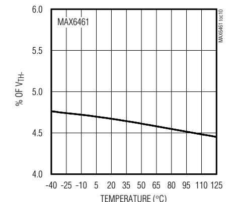
HYSTERESIS vs. TEMPERATURE
