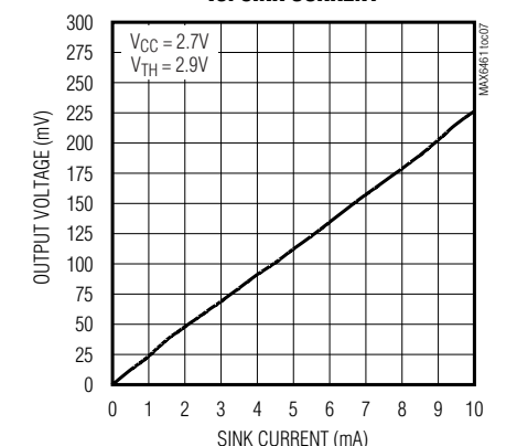
OUTPUT VOLTAGE LOW vs. SINK CURRENT
