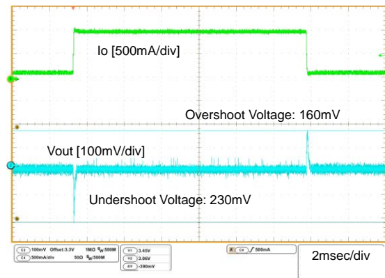
Fig.24 Load Response Iout:100mA \leftrightarrow 1A
