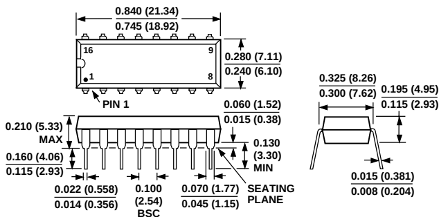
16-Lead Plastic (N-16)
