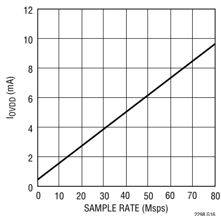
LTC2298: I_{VDD} vs Sample Rate, 5MHz Sine Wave Input, -1dB, O_{VDD} = 1.8\text{V}
