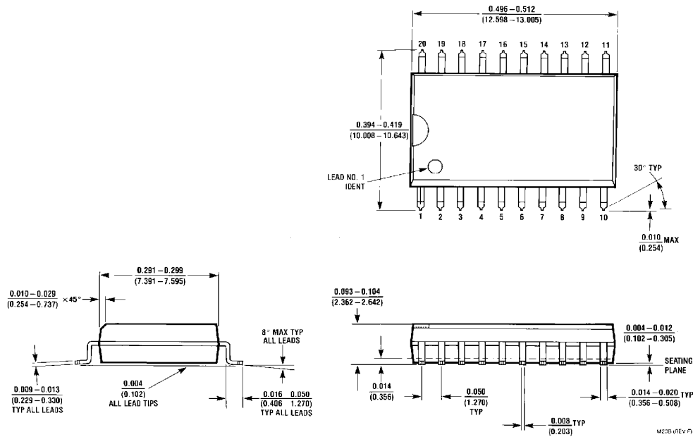
S.O. Package (M) Order Number DM74ALS534M Package Number M20B
