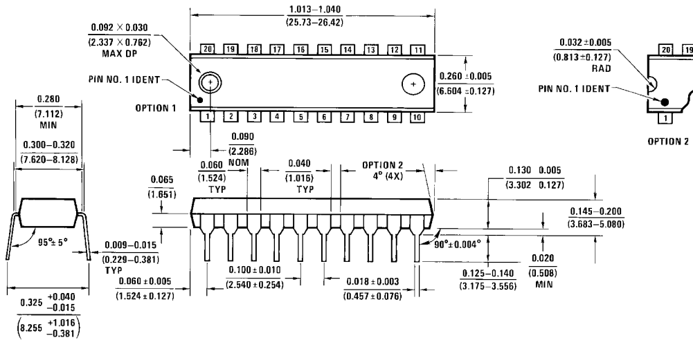
Molded Dual-In-Line Package (N) Order Number DM74ALS534N Package Number N20A
