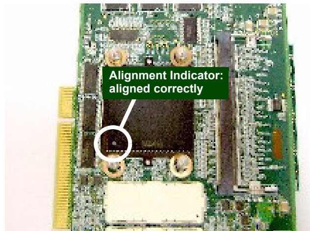
Figure 7-16. Chip alignment: Correct
