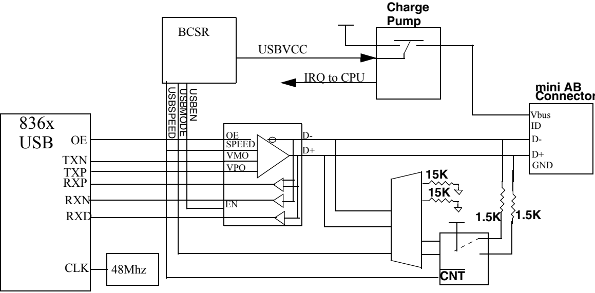
Figure 5-15. USB 1.1 Block
