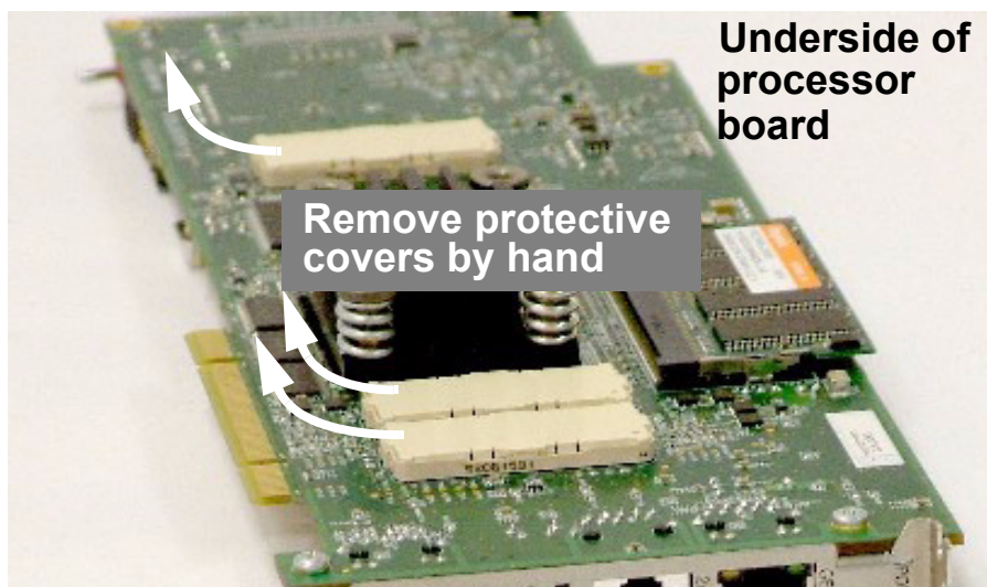
Figure 2-3. Remove Protective Covers from 300-pin connectors (underside of MPC8360 MDS Processor Board shown)
