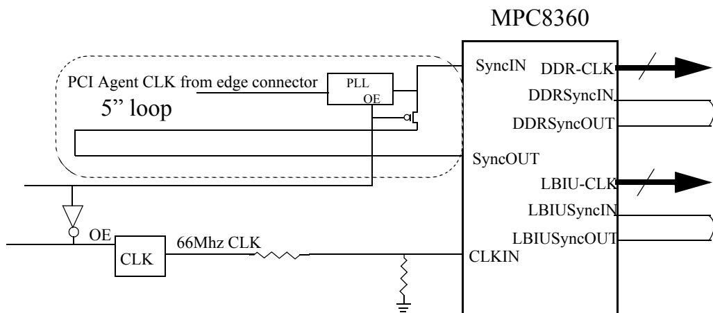
Figure 5-4. Clocks - Showing External Connection Scheme, and 5'' Loop
