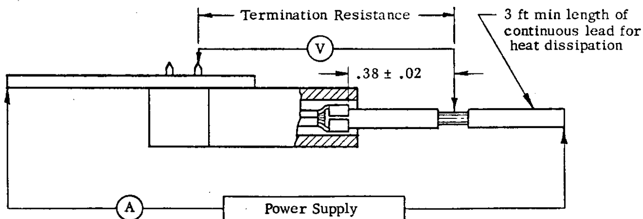
Termination Resistance Test Circuit
