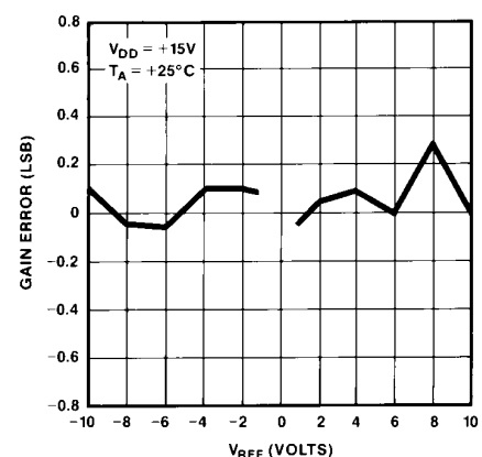
Absolute Gain Error Change vs. V_{REF}
