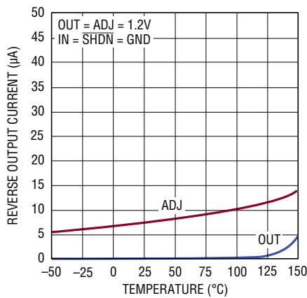
Reverse-Output Current
