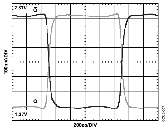
Figure 7. Output Waveform, V_{CC} = 3.3\text{ V}
