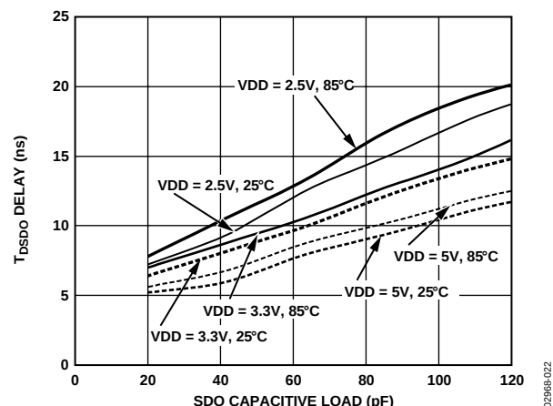
Figure 23. t_{DSO} vs. Capacitance Load and Supply
