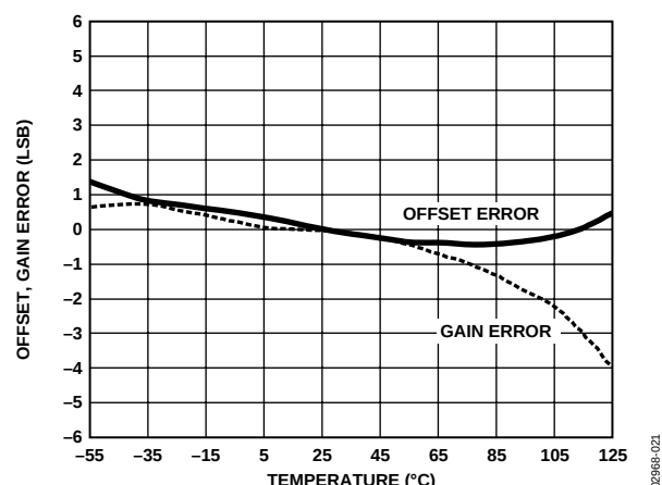
Figure 22. Offset and Gain Error vs. Temperature
