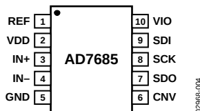
Figure 5. 10-Lead MSOP and QFN¹ (LFCSP) Pin Configuration
