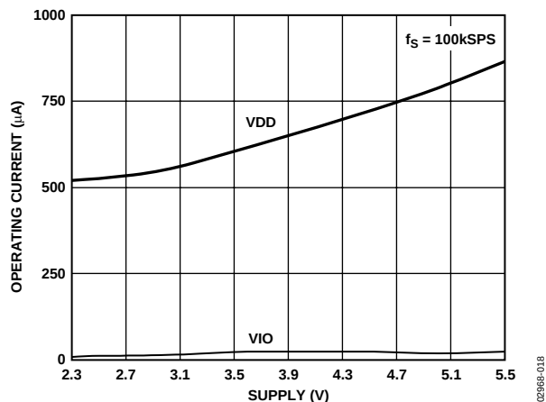
Figure 19. Operating Currents vs. Supply
