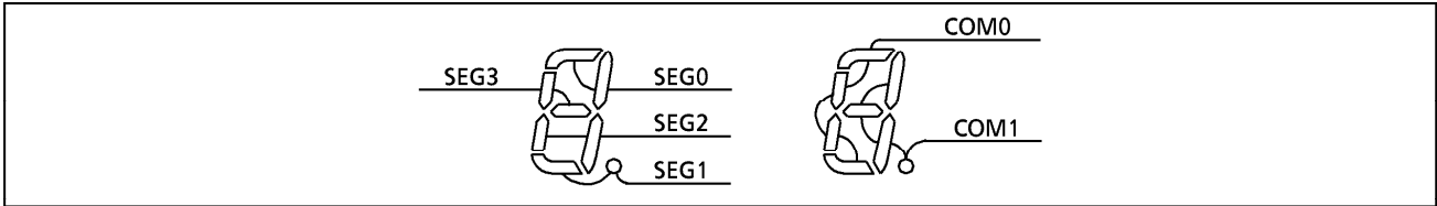
Figure 2-48. Example of COM, SEG Pin Connection
