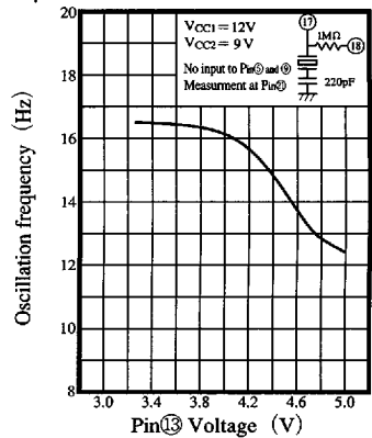
\beta Characteristics of Horizontal Oscillator
