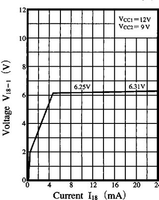
Zener Characteristics (1)
