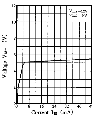
Zener Characteristics (2)
