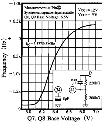
\beta Characteristics of Chroma Oscillator
