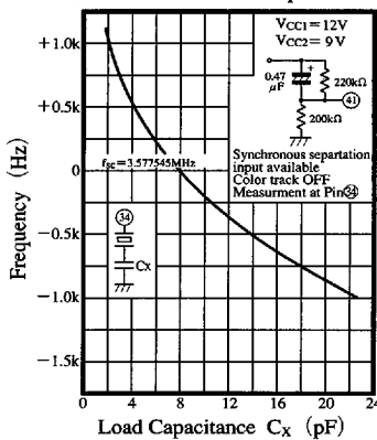
Fluctuation of Oscillation Frequency (fsc) vs. that of Load capacitance
