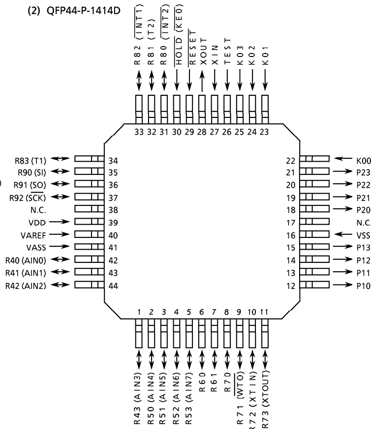
(2) QFP44-P-1414D
