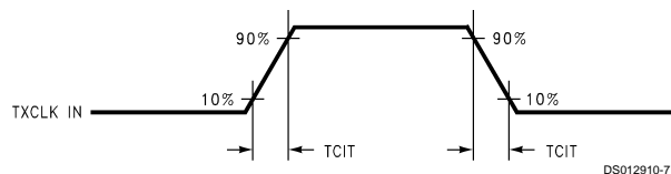
FIGURE 4. DS90CR285 (Transmitter) Input Clock Transition Time
