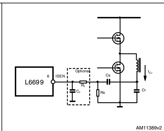
Figure 19. Current sensing techniques “lossless”, with capacitive shunt
