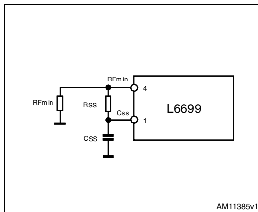
Figure 12. Soft-start circuit
