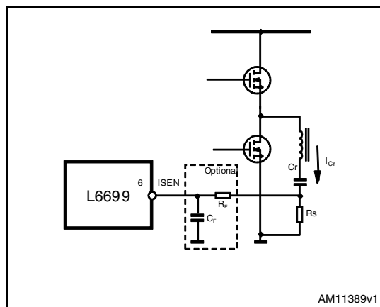
Figure 18. Current sensing techniques with sense resistor
