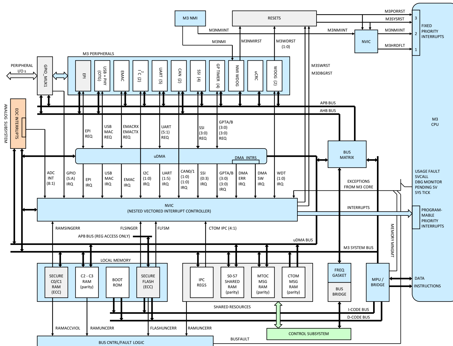
Figure 6-1. Master Subsystem
