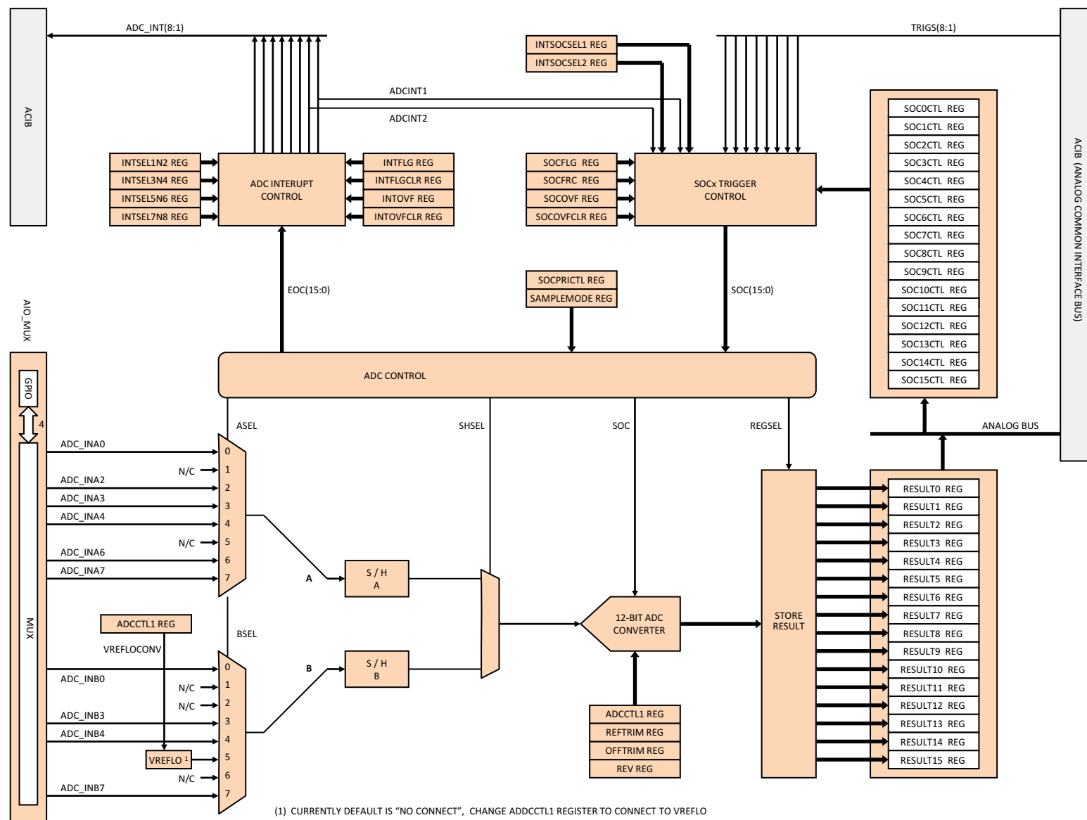
Figure 5-11. ADC
