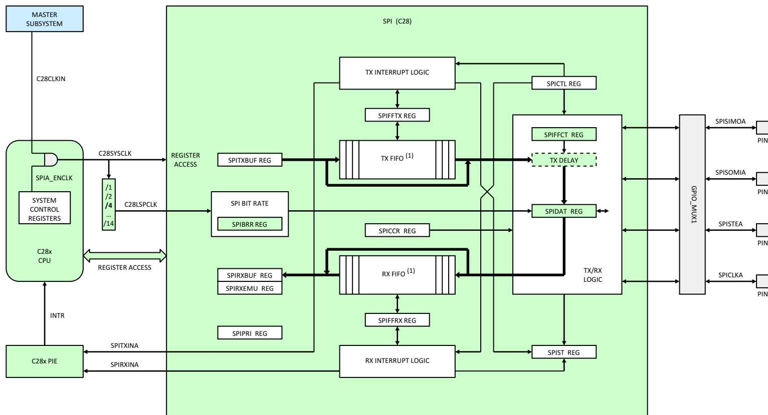
Figure 5-51. SPI (C28x)
