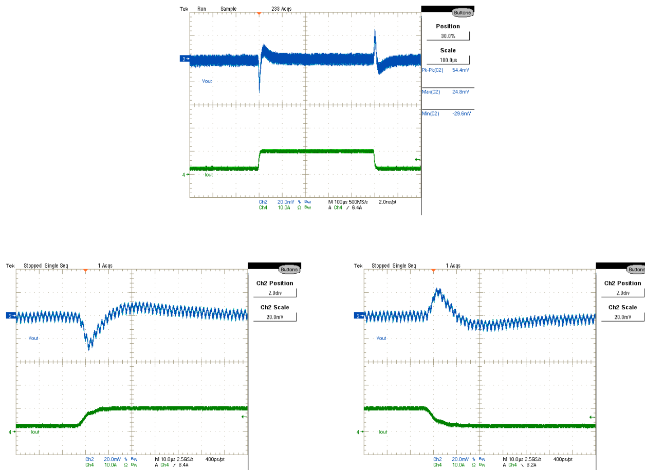
Figure 37: Vout Transient Response, 2.5A to 10.0A step at 2.5A/µSec CH2:Vout, CH4:Iout (10A/V)
