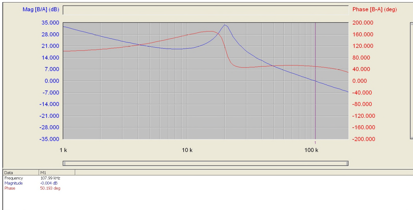
Figure 39: Bode Plot with 25A load: Fo=108 kHz, Phase Margin=50.2 Degrees
