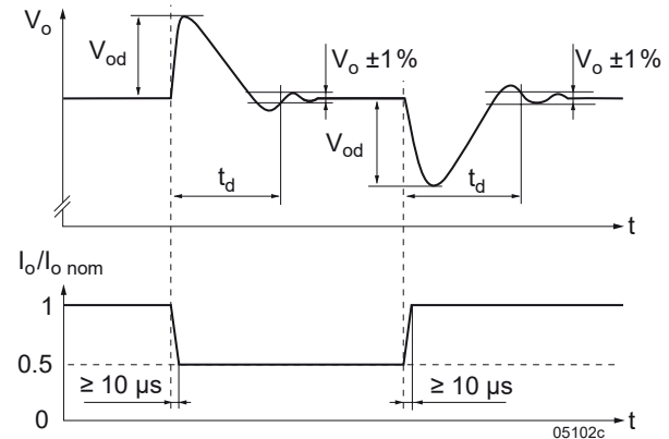
Fig. 14 Typical dynamic load regulation of V_o .
