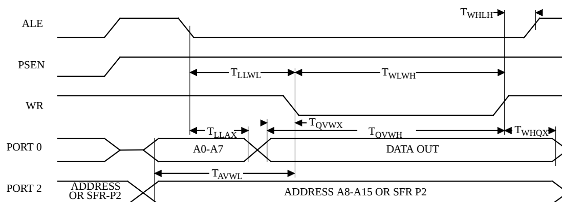
Figure 15. External Data Memory Write Cycle
