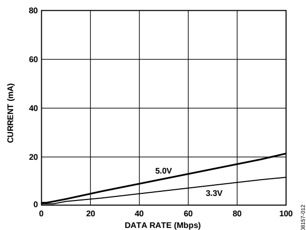
Figure 12. Typical ADuM4400 V_{DD2} Supply Current vs. Data Rate for 5 V and 3.3 V Operation
