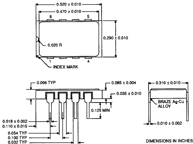
8-Pin Ceramic Sidebrazed DIP (CD8)
