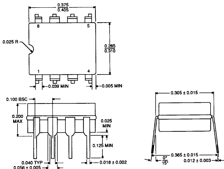
8-Pin CerDIP (DD8)
