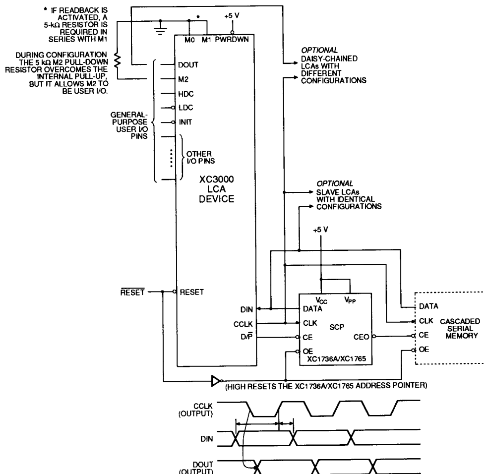
Figure 2. Master Serial Mode. The one-time-programmable XC1736A/XC1765 Serial Configuration PROM supports automatic loading of configuration programs up to 36K/64K bits. Multiple devices can be cascaded to support additional LCAs. An early D/\bar{P} inhibits the PROM data output a CCLK cycle before the LCA I/Os become active.
