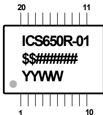
Marking Diagram—ICS650R-01
