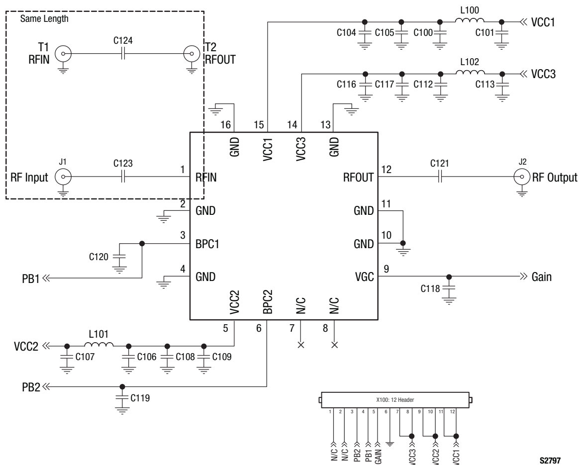
Figure 6. SKY65373-11 Evaluation Board Schematic
