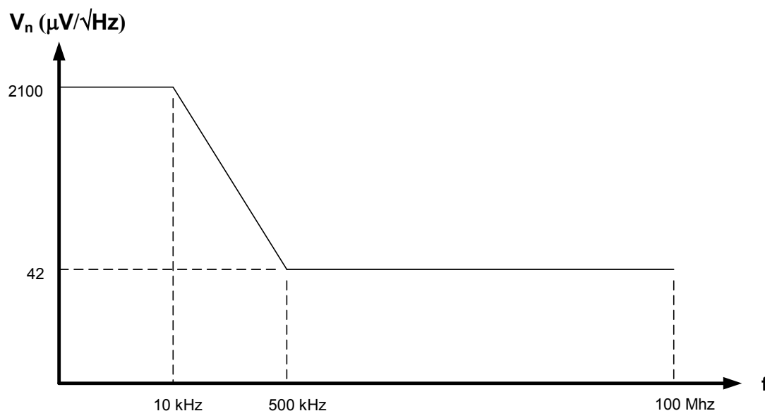
Figure 9. Power Supply Noise Tolerance Mask
