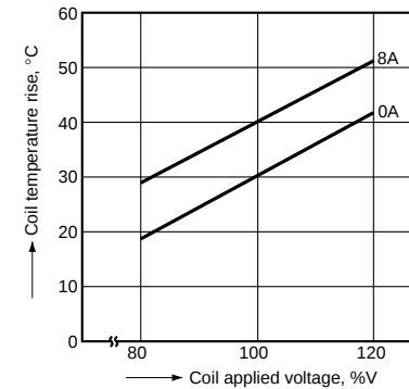
3.-(1) Coil temperature rise (1 Form A) Tested sample: DSP1a-DC12V, 5 pcs.
