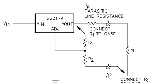
Figure 18 – Connections for Best Load Regulation
