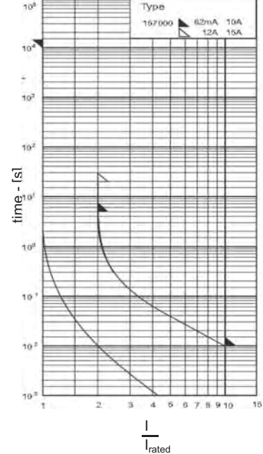
Time-Current Characteristics
