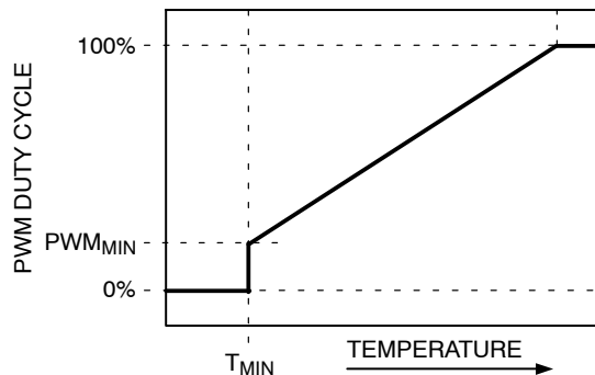
Figure 50. PWM_{MIN} Determines Minimum PWM Duty Cycle
