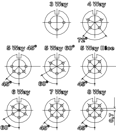
PCB DRILLING - ALL PIN HOLES Ø1.2mm ON A 7.00 P.C.D.
