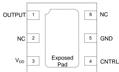
U-DFN2020-6
