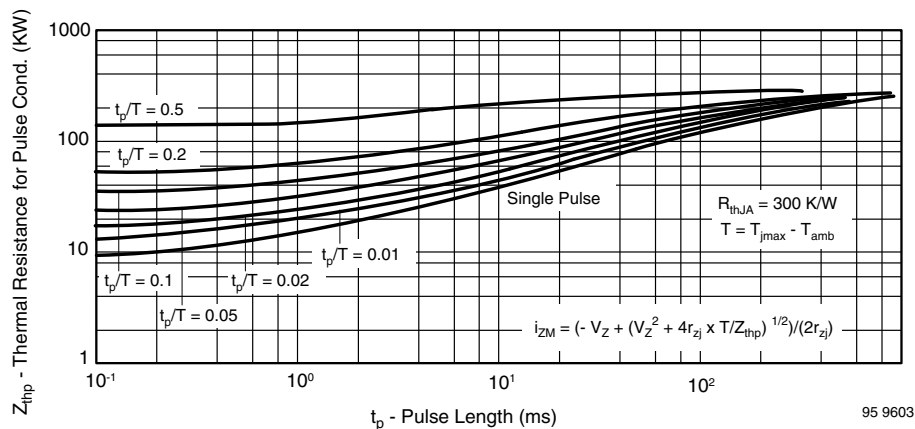
Fig. 13 - Thermal Response
