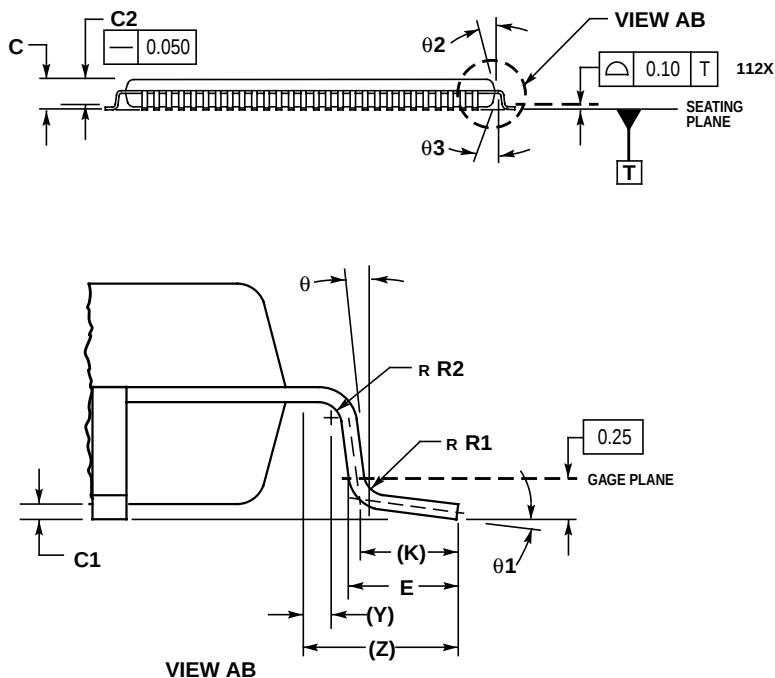
Figure B-1 112-pin LQFP mechanical dimensions (case no. 987)
