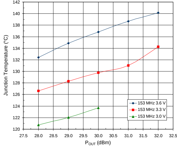
RF5110G 153 MHz Junction Temperature Versus P_{OUT}/V_{CC} Ambient Temperature = 85°C
