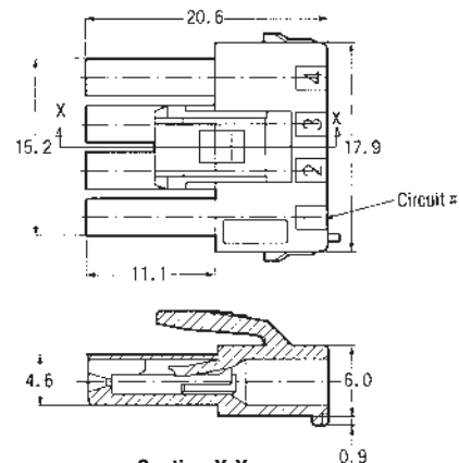
Section X-X
