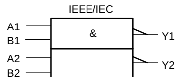
Figure 2. Logic Symbol
