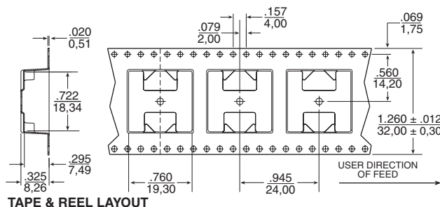
TAPE & REEL LAYOUT
