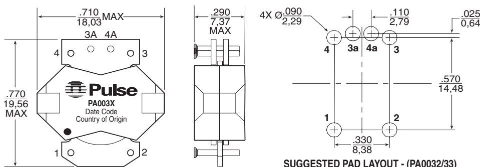
SUGGESTED PAD LAYOUT - (PA0032/33)
