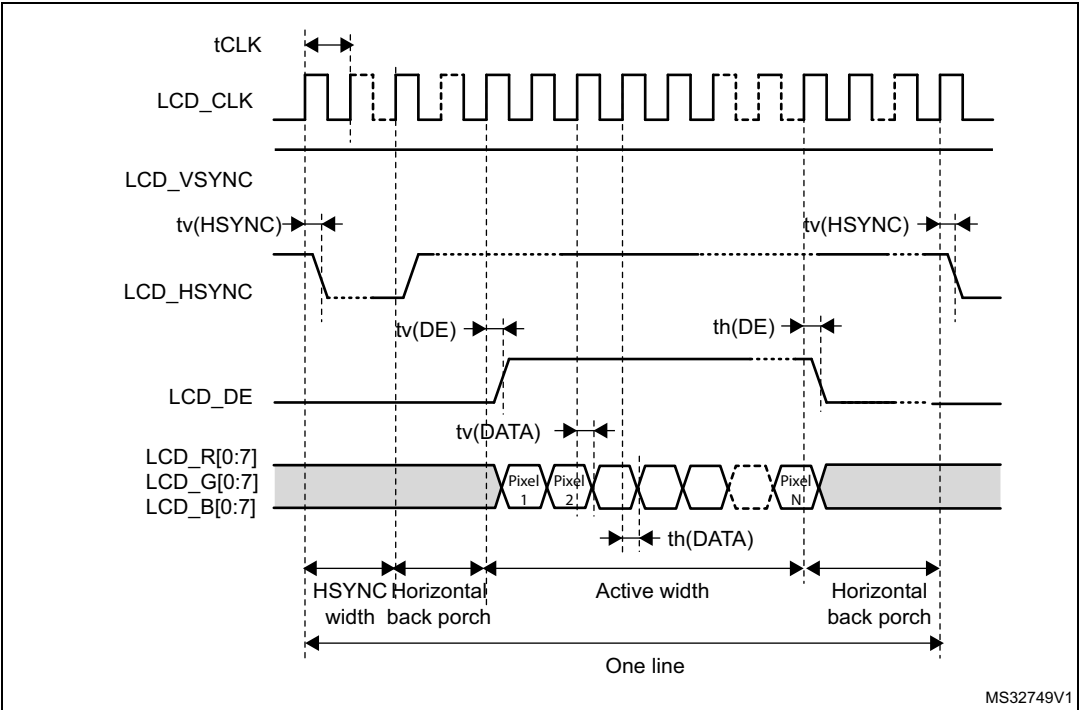
Figure 49. LCD-TFT horizontal timing diagram
