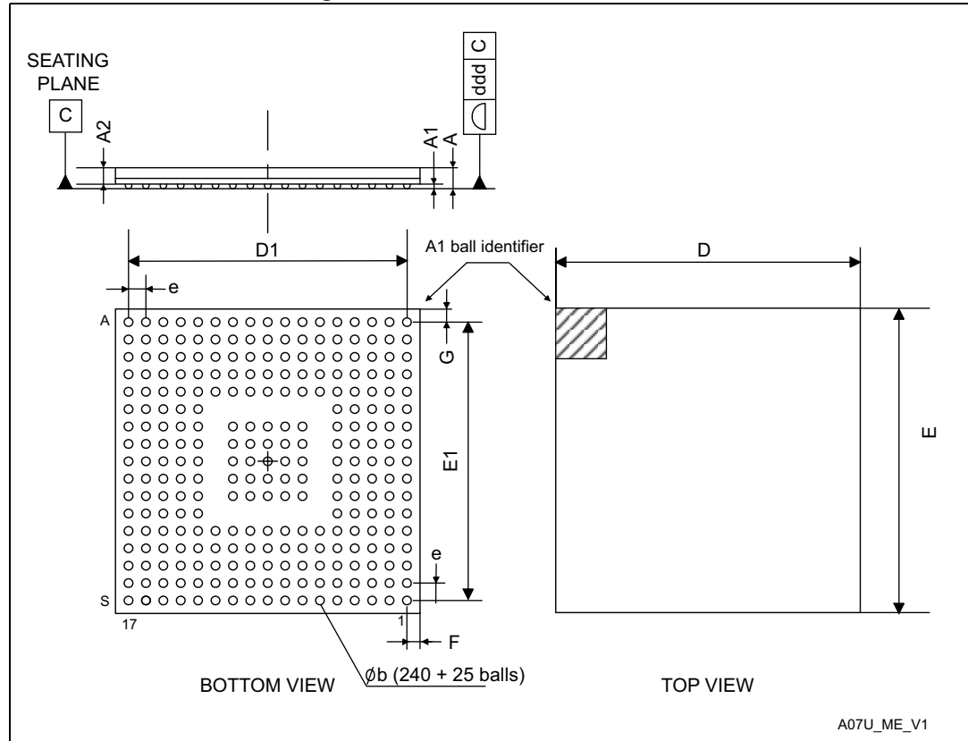
Figure 78. TFBGA240+25 - Outline
