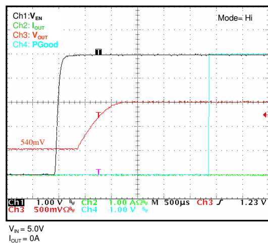
Start Up into Pre-Biased Output ( V_{OUT}=1.5V )
