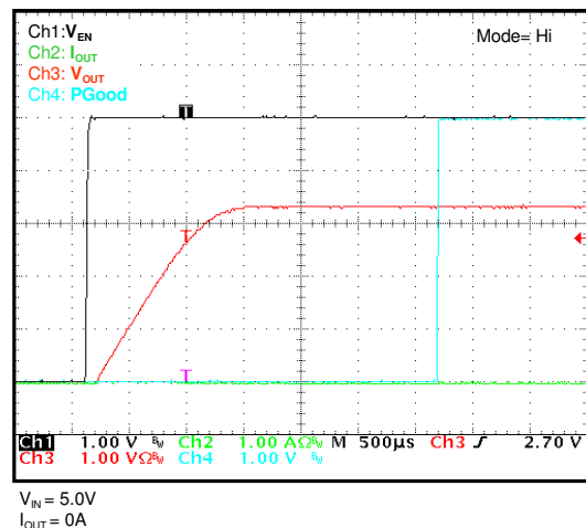
Start Up (Enable) ( V_{OUT}=3.3V ), forced PWM
