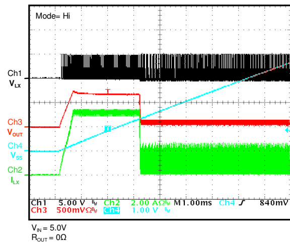
Start Up (Enable) into Output Short Circuit
