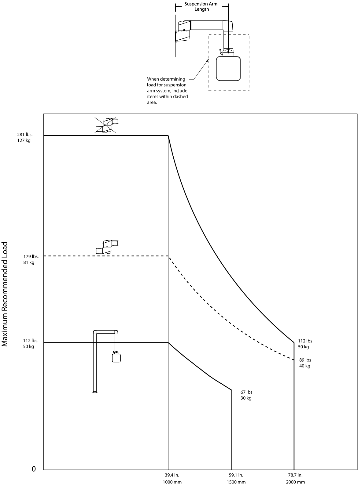
Load Diagram
