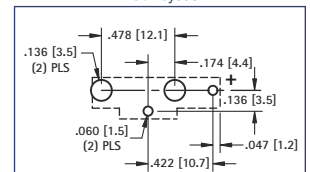
Pad Layout
