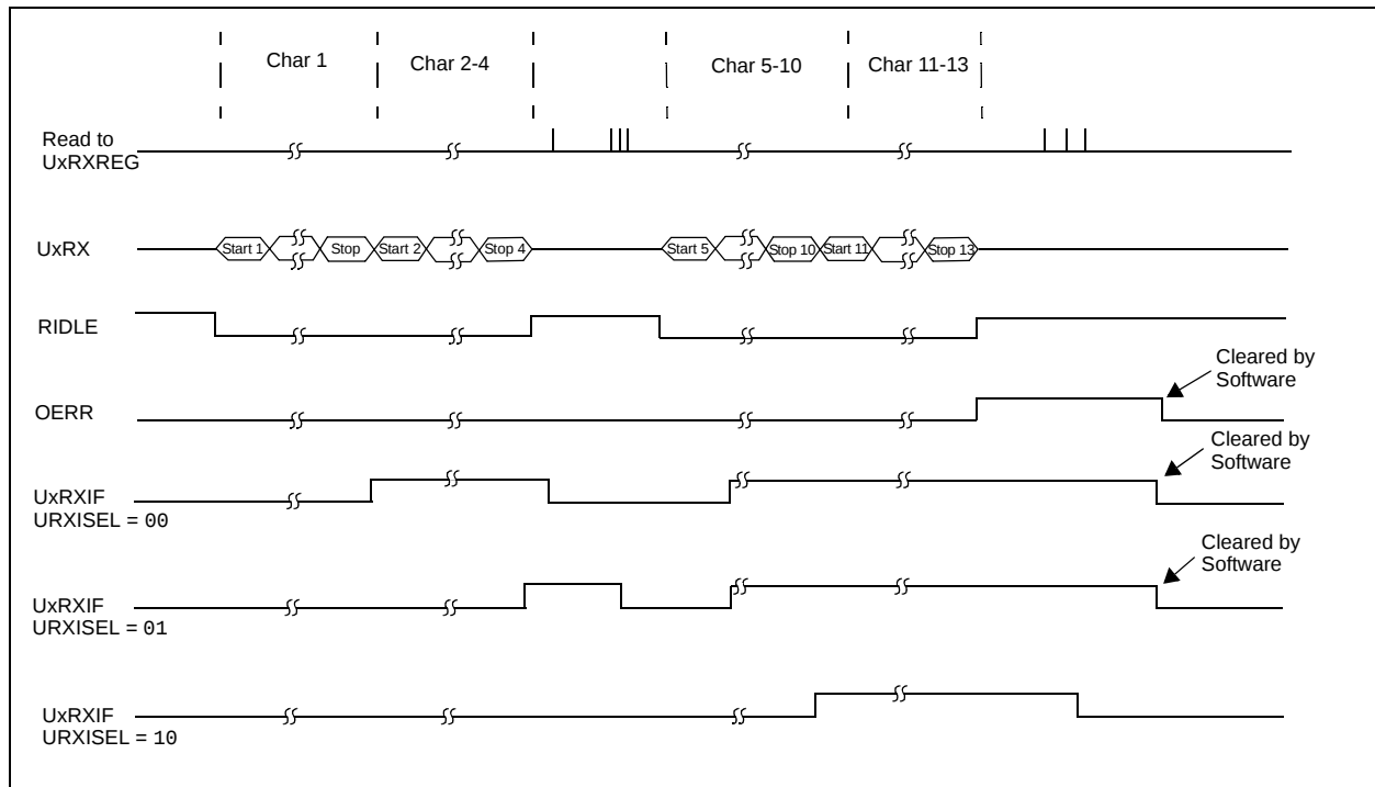
FIGURE 19-2: UART RECEPTION
