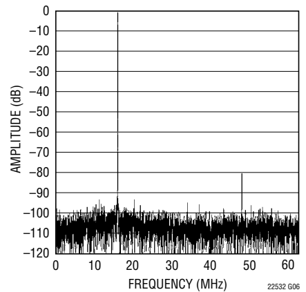
LTC2253: 8192 Point FFT, f_{IN} = 140\text{MHz} , -1dB, 2V Range, 125Msps
