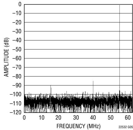
LTC2253: 8192 Point FFT, f_{IN} = 70\text{MHz} , -1dB, 2V Range, 125Msps
