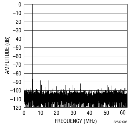
LTC2253: 8192 Point FFT, f_{IN} = 5\text{MHz} , -1dB, 2V Range, 125Msps
