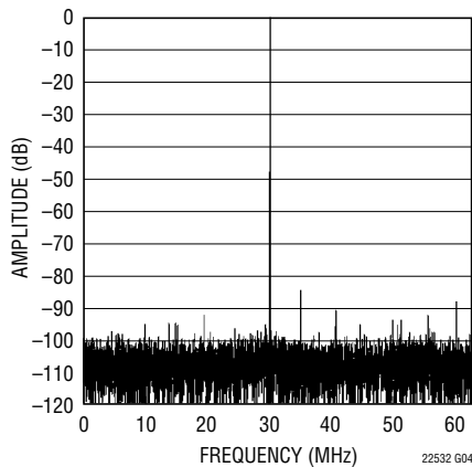
LTC2253: 8192 Point FFT, f_{IN} = 30\text{MHz} , -1dB, 2V Range, 125Msps
