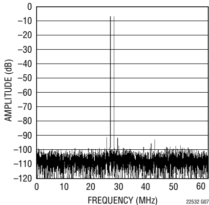
LTC2253: 8192 Point 2-Tone FFT, f_{IN} = 28.2\text{MHz} and 26.8\text{MHz} , -1dB, 2V Range, 125Msps
