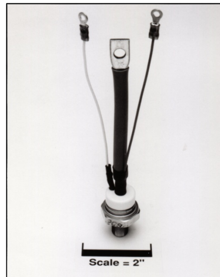
2N4361-2N4371 Phase Control SCR 70 Amperes Average (110 RMS), 1400 Volts
