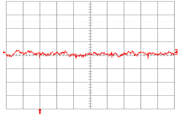
Fig. 1.5V.14: Input reflected-ripple current, i_s (10 mA/div.), measured through 10 μH at the source at full rated load current and V_{in} = 48 V. Refer to Fig. 1.5V.12 for test setup. Time scale: 1 μs/div.
