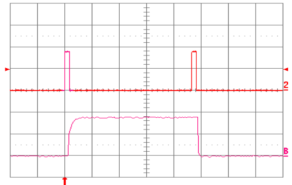
Fig. 1.5V.16: Load current (top trace, 20 A/div., 50 ms/div.) into a 10 mΩ short circuit during restart, at V_{in} = 48 V. Bottom trace (20 A/div., 2 ms/div.) is an expansion of the on-time portion of the top trace.
